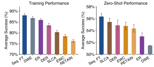
Figure 4: Averaged across three benchmarks, Seq. FT obtains strong performance in both performance (AVG) and generalization (ZS).
