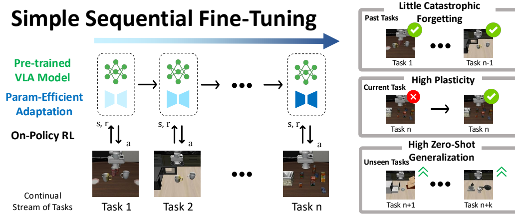
Figure 1: VLAs as Natural Continual Learners. We show that the synergy between pre-trained VLA, on-policy RL, and LoRA is enough to overcome catastrophic forgetting while maintaining plasticity, enabling simple Sequential Fine-Tuning to achieve surprisingly good performance.
