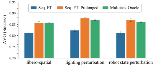
Figure 7: Final training success rates: by simply prolonging the Seq. FT training steps, we can obtain on-par performance with multitask oracle.
