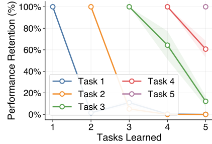
Figure 5: VLA, on-policy RL, and LoRA are all crucial to stability. Removing any one of them results in catastrophic forgetting, shown by the curve.
