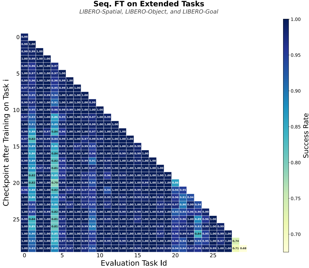
Figure 6: Performance on tasks after sequentially training on 30 tasks. Seq. FT remains robust under extended length of the training task sequence.
