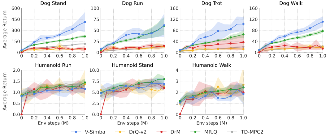
Figure 5: DeepMind Control Suite - Hard. Average episode returns on 7 hard-level tasks from DeepMind Control Suite (Tassa et al., 2018). Each curve represents the mean performance across 5 random seeds per algorithm; shaded areas indicate 95% bootstrap confidence intervals.
