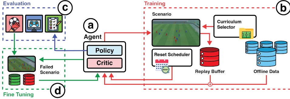
Figure 2: Overview of the proposed method. (a) shows the agent composed of the policy and action-value functions as employed by SAC. (b) shows the main training framework, composed of the elements delineated in Section 3.3: curriculum learning , offline data , and network resets . (c) shows the three components of the evaluation framework: automatic quantitative evaluation , human qualitative evaluation , and expert-authored test suite , described in Section 3.6. Finally, (d) shows the fine tuning component. In this, we use only the failed scenario to generate new data but we combine it with the previously collected replay buffer. More details in Section 3.7.
