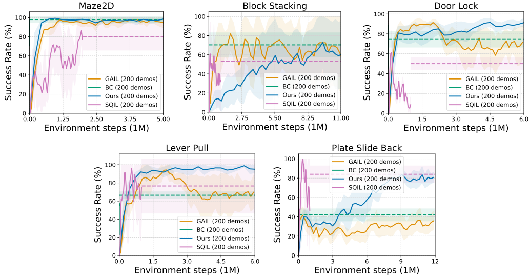
Figure 9: Comparison of MPG with traditional IL and IRL approaches in a standard IL setting with ample demonstrations.
