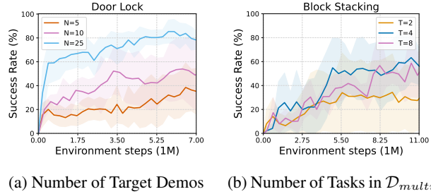
Figure 4: Data efficiency analysis. Effect of (a) demonstration quantity and (b) task diversity.
