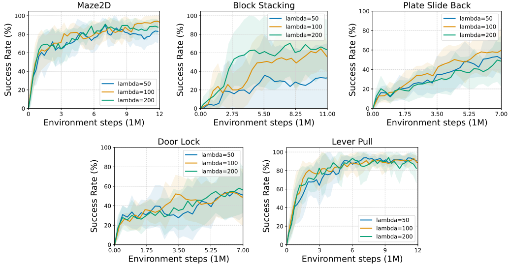
Figure 11: Analysis on \lambda , the coefficient of the proximity reward, in more tasks.
