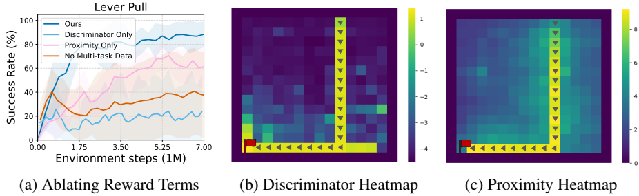
Figure 5: Ablation of MPG's reward components.
