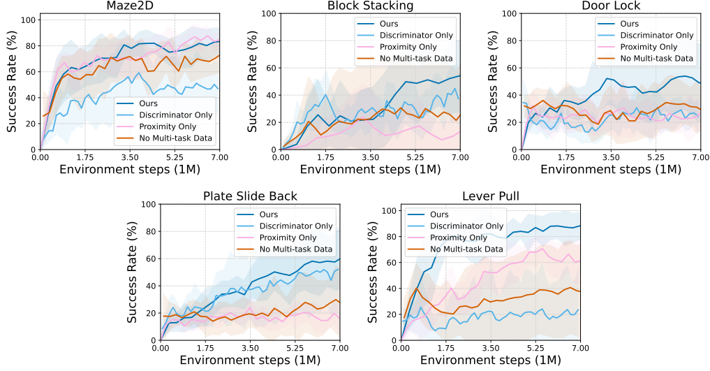
Figure 10: Ablations over more tasks in supplement to Figure 5
