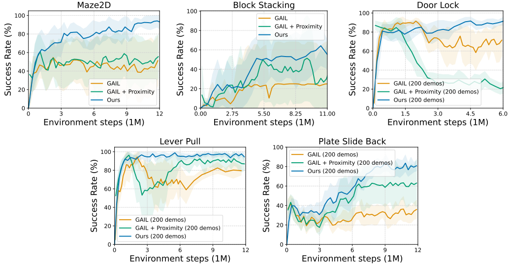
Figure 13: Analysis of our proximity reward by combining it with GAIL without multi-task data (GAIL + Proximity).
