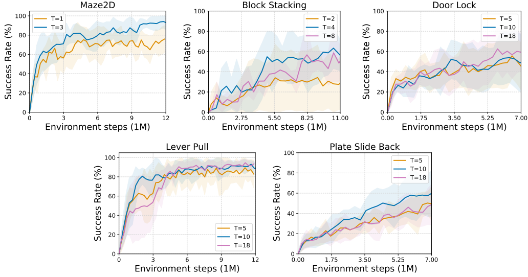
Figure 8: Analysis on the number of tasks in the multi-task dataset in more tasks.
