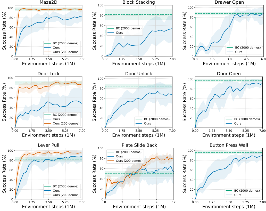
Figure 6: Comparisons with an “oracle” BC method given 2000 demonstrations.
