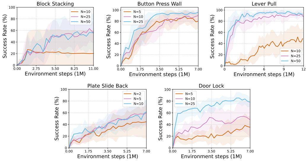
Figure 7: Analysis on the number of target task demonstrations in more tasks.
