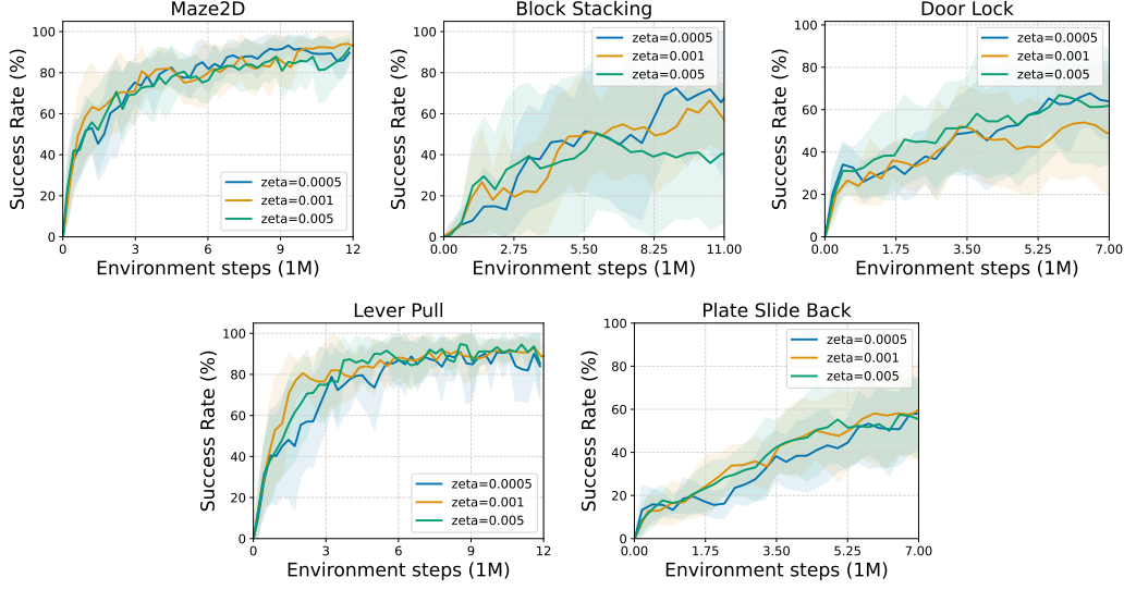
Figure 12: Analysis on zeta \zeta , the proximity timestep factor, in more tasks.
